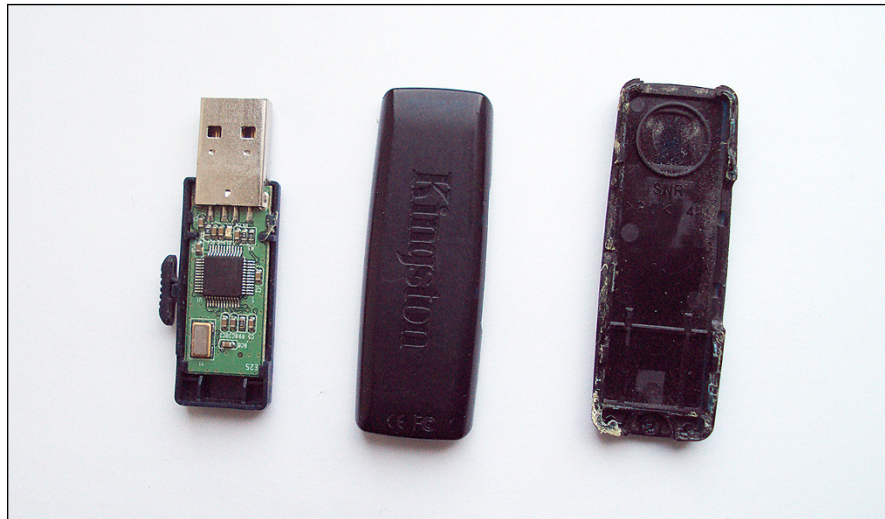
FIGURE 1-10: The inside of a USB drive.
