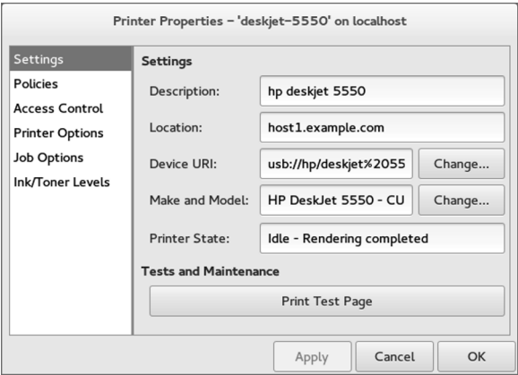
FIGURE 16.3 The Printer Properties window after adding a printer
