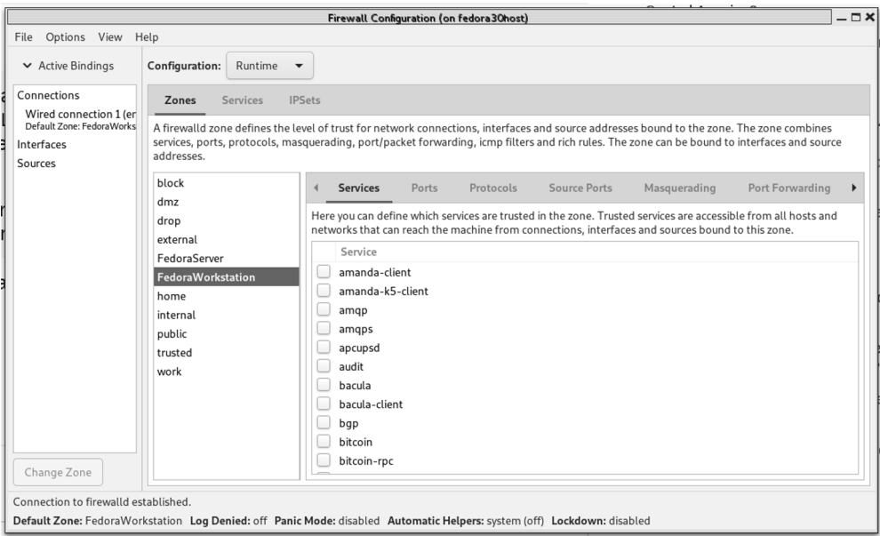
FIGURE 25.1 Firewall Configuration window
