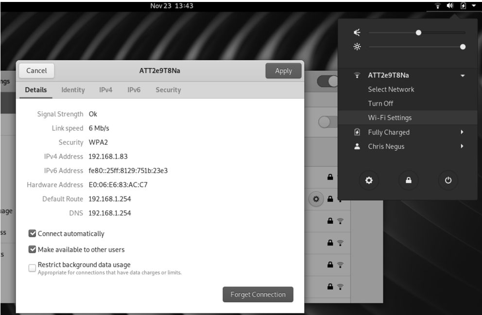
FIGURE 14.1 Checking network interfaces with NetworkManager
