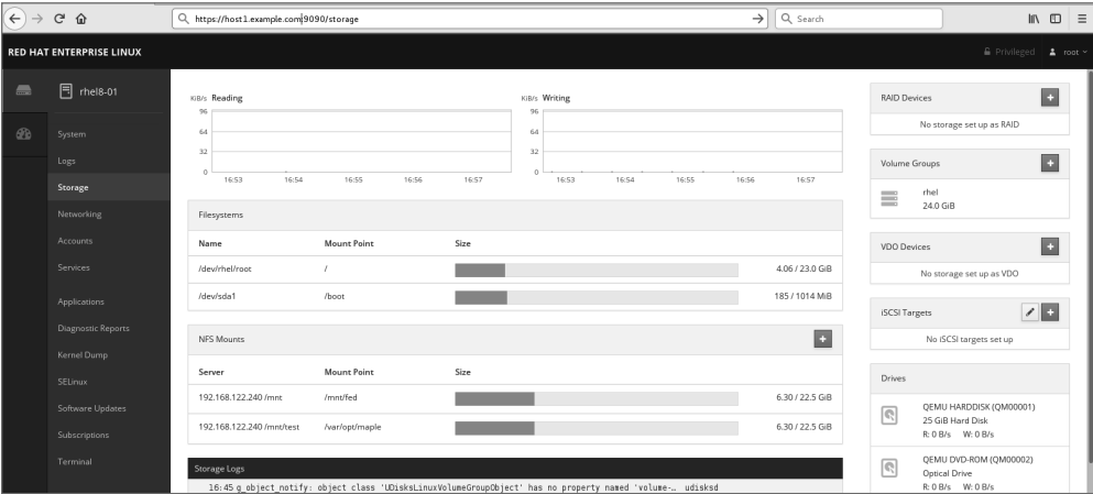
FIGURE 20.2 Add a new NFS mount using Cockpit Web UI
