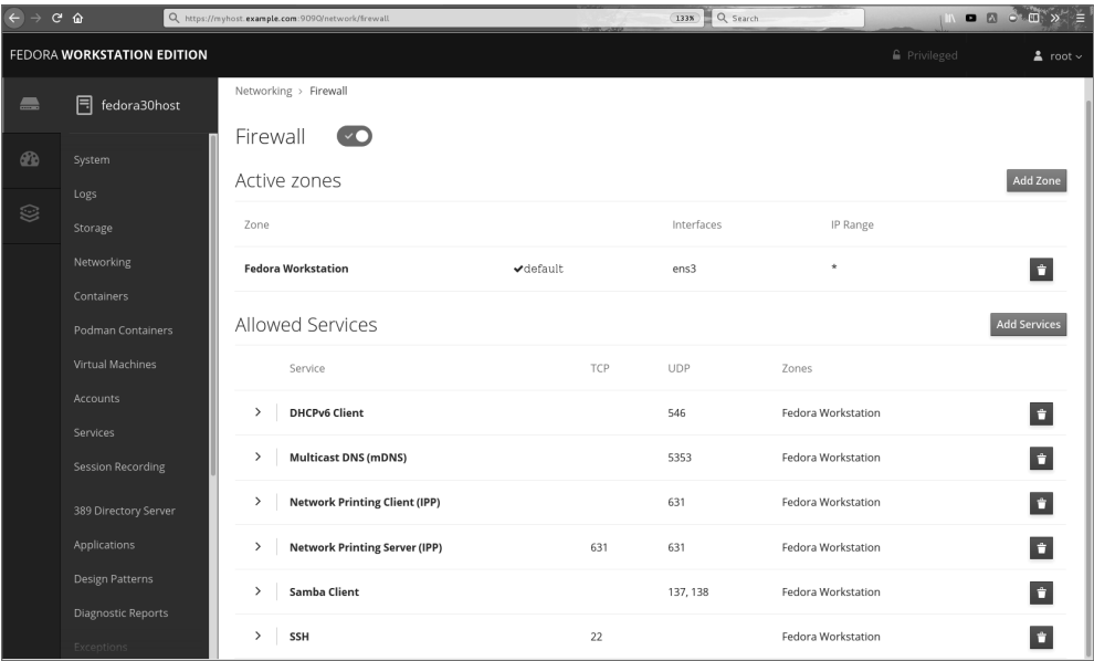
Firewall Configuration
