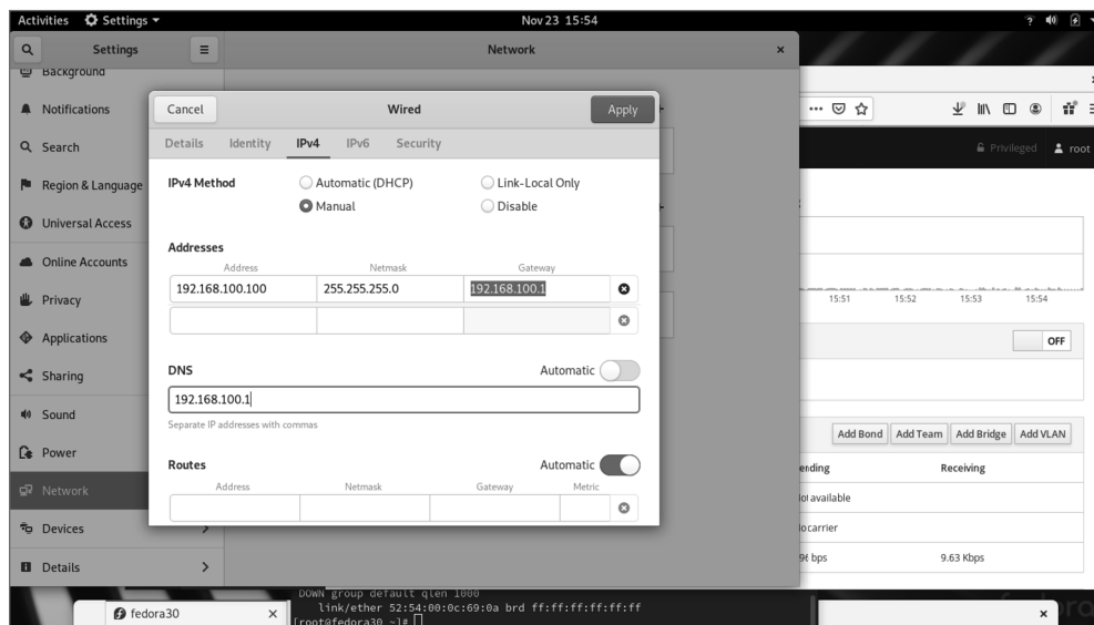
FIGURE 14.5 Changing network settings with NetworkManager
