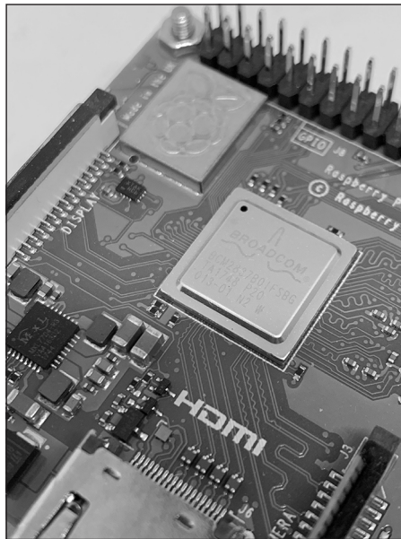
FIGURE 4-1: The Raspberry Pi processing chip containing the Videocore-IV.
