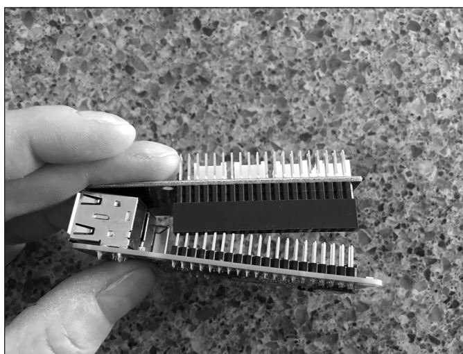
FIGURE 1-5: Aligning the Pi2Grove board with the Raspberry Pi.
